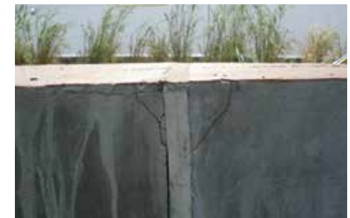
Concrete Planter Damage
